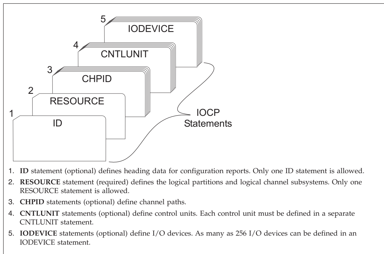
Figure 16. IOCP statements
